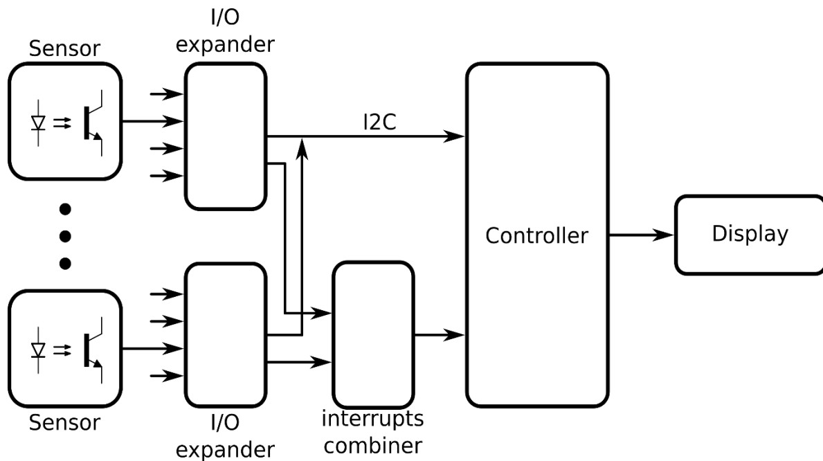
FIGURE 2. Block diagram of the electronics system.
