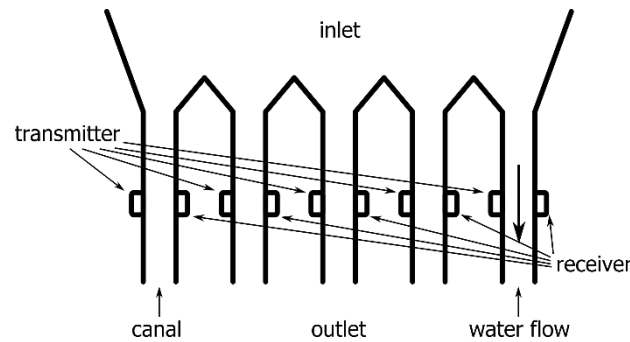
FIGURE 4. Fry counting mechanism.
