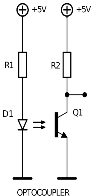
FIGURE 1. Opto-coupler sensor schematic.
