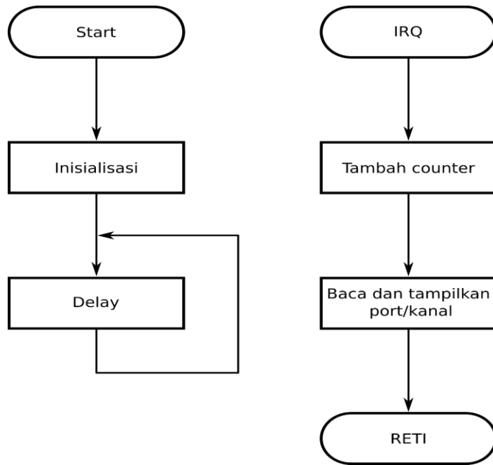
FIGURE 3. Flowchart of software of fry counter system.
